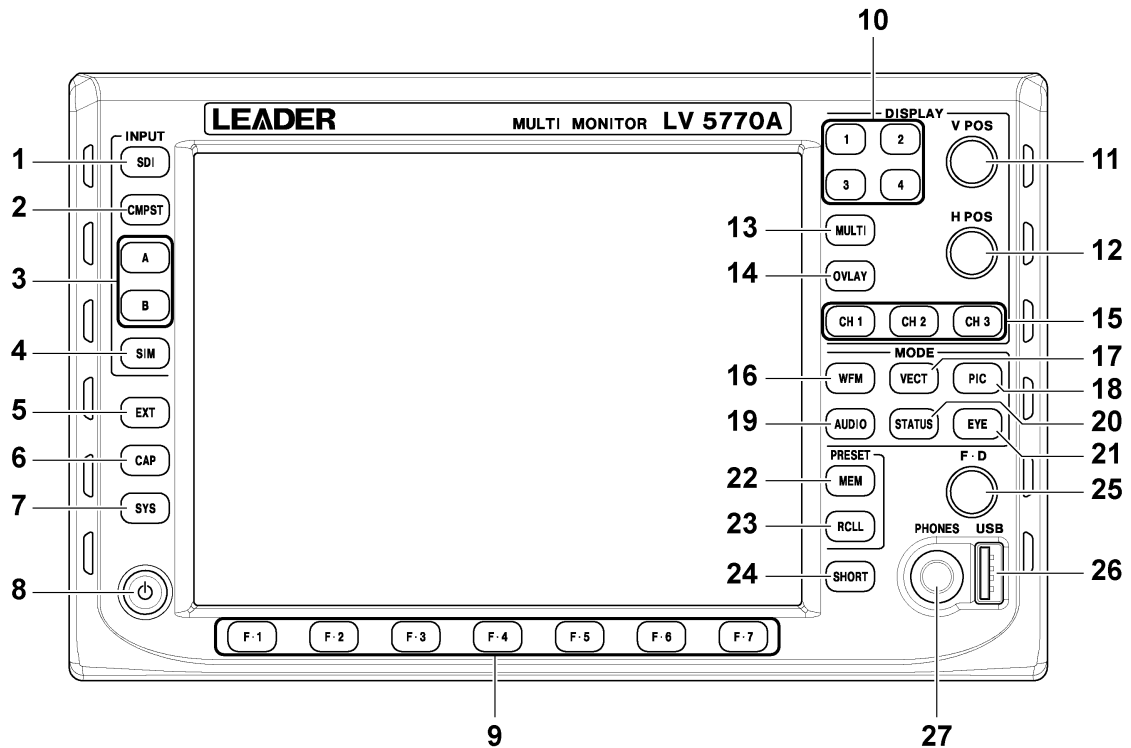
Figure 3-1 Front panel
