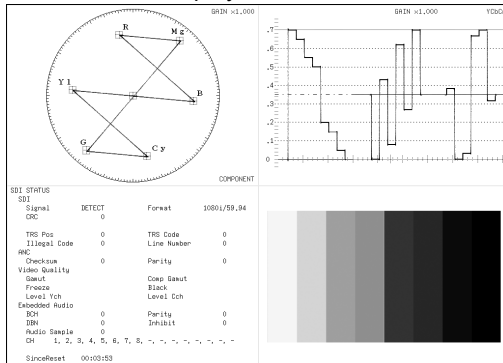
4-screen multi display
