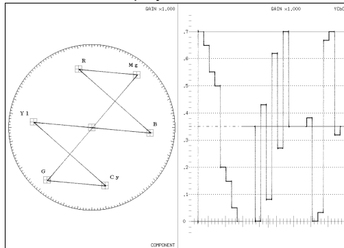
2-screen multi display
