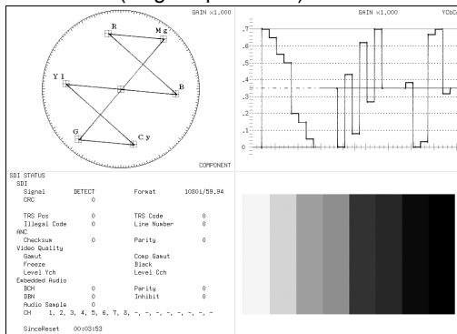
SIM = OFF (single input mode)
