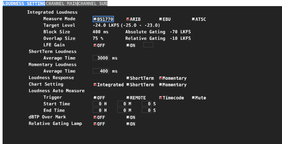
Figure 13-33 LOUDNESS SETTING tab
