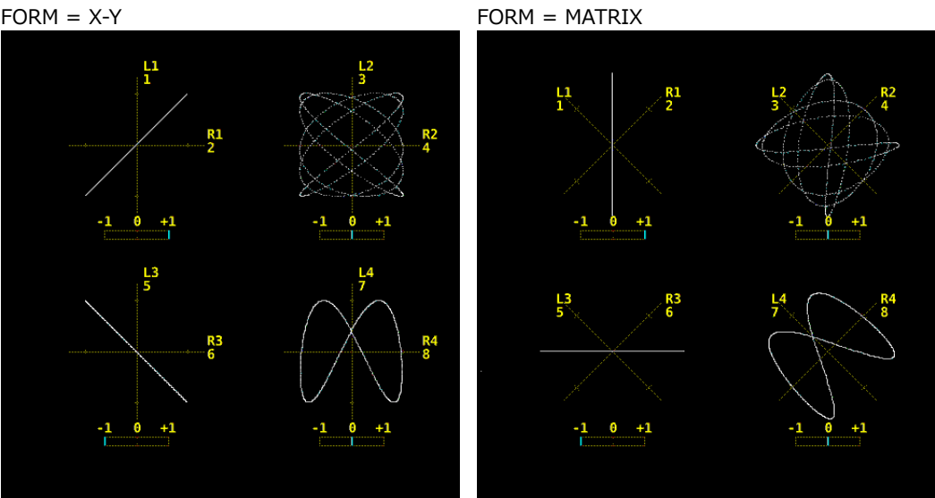
Figure 13-13 Selecting the scale display format
