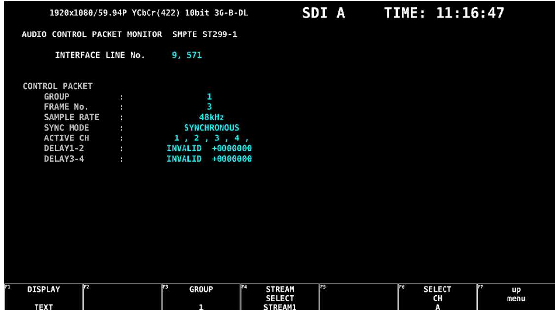
Figure 14-17 Audio control packet screen
