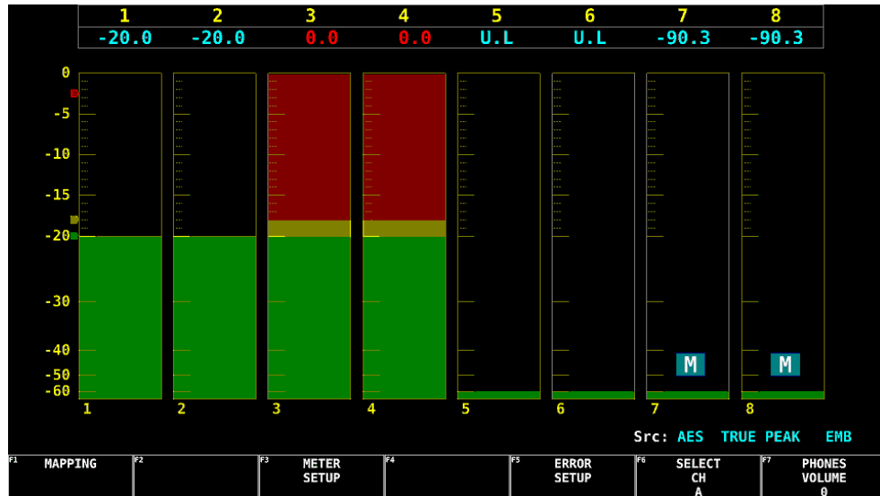
Figure 5-21 Audio display
