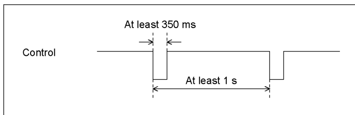
Figure 18-3 Control timing 1
