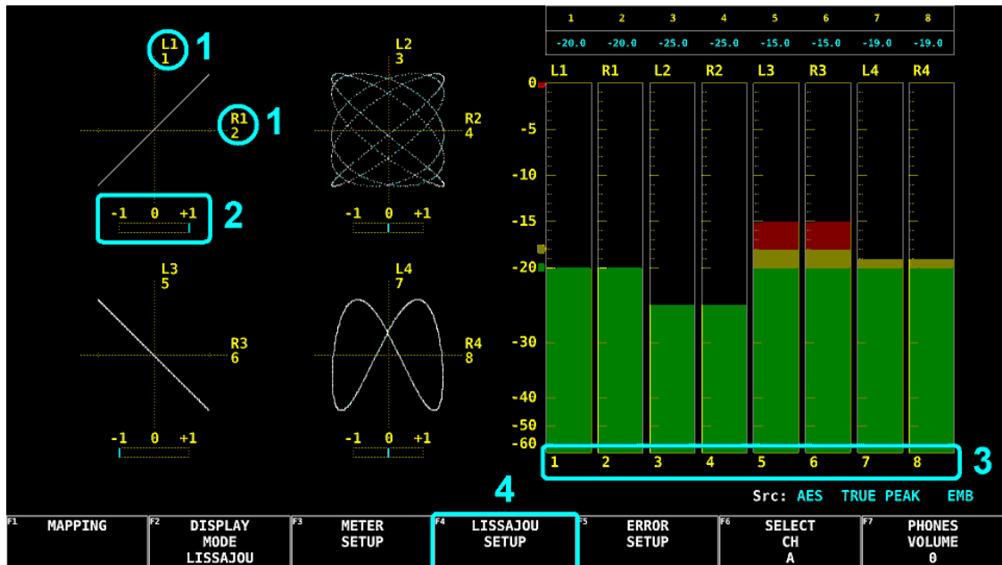
Figure 13-10 Lissajous display
