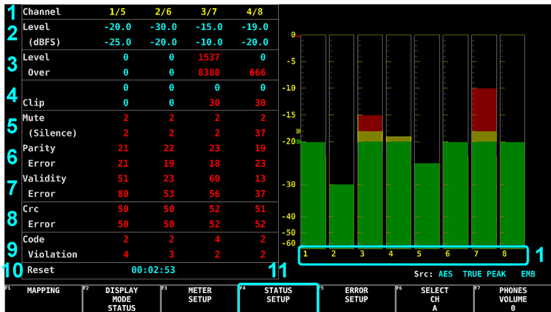
Figure 13-18 Status display
