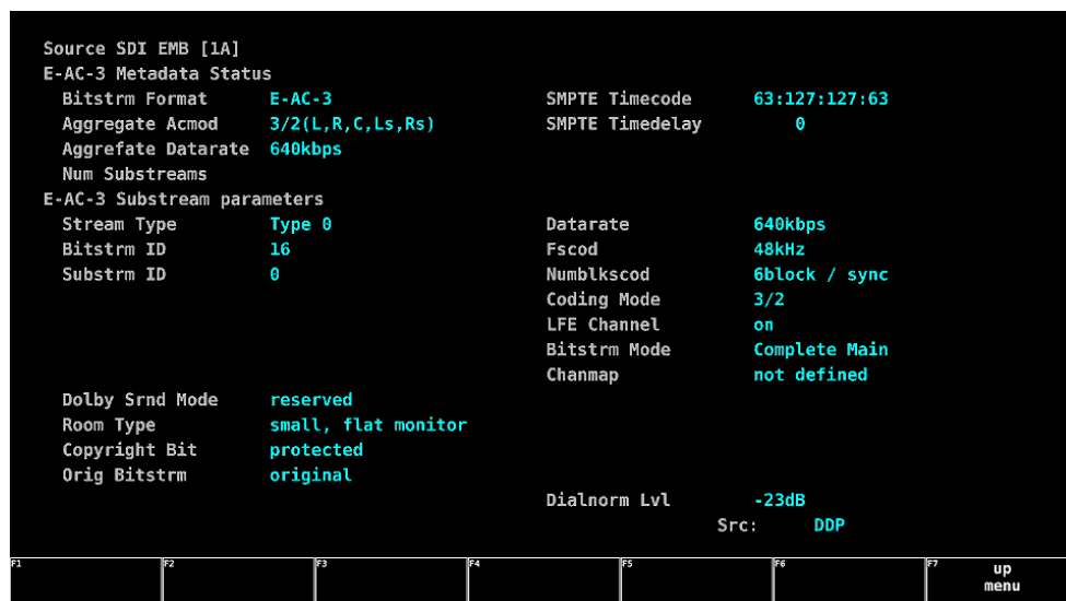
Figure 13-26 Dolby Digital Plus Metadata display
