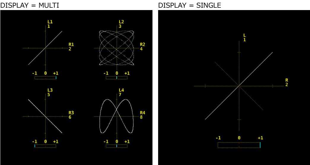
Figure 13-12 Selecting the Lissajous curve display format
