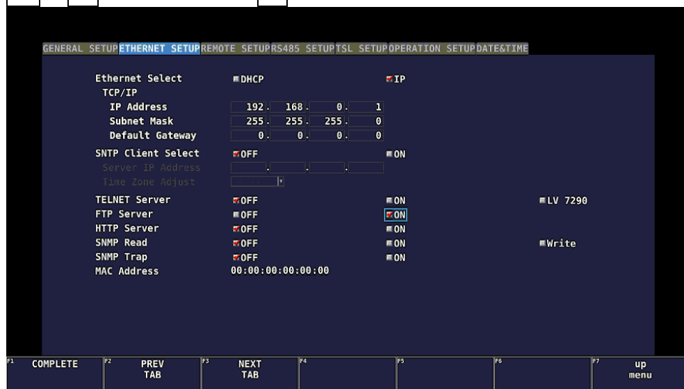
Figure 17-4 ETHERNET SETUP tab
