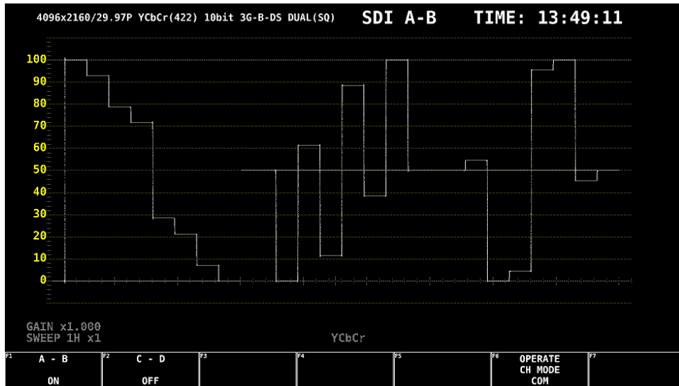
Figure 5-11 Measurement screen
