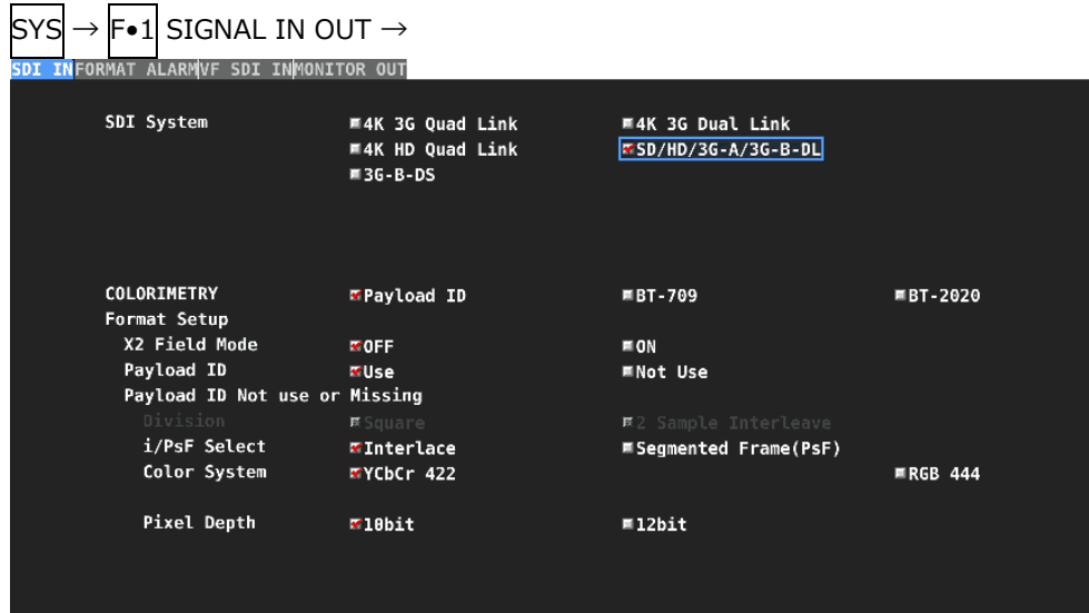
Figure 5-3 SDI IN tab
