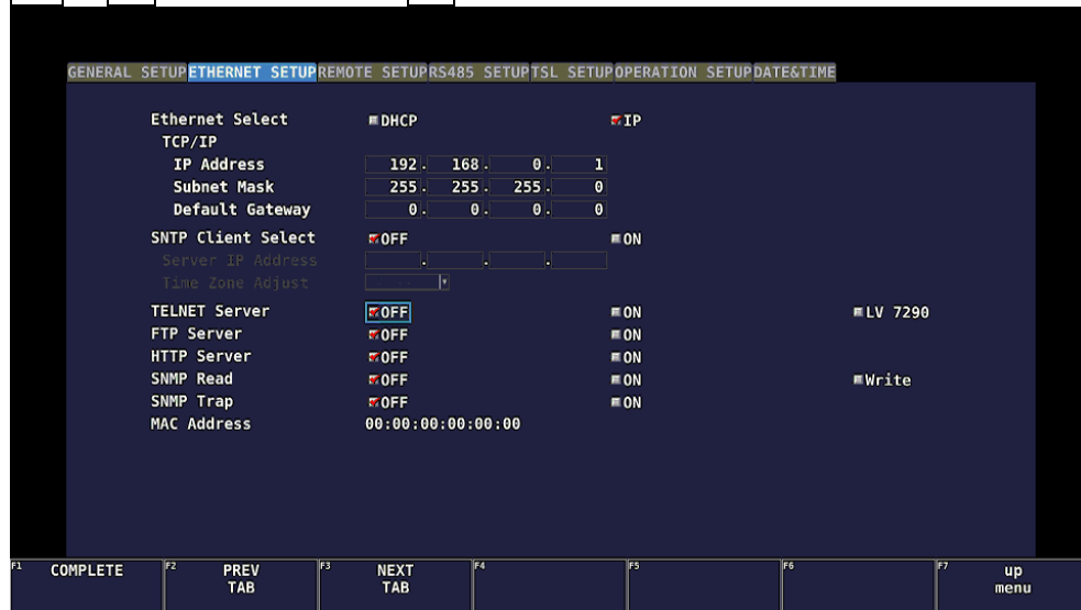
Figure 6-9 ETHERNET SETUP tab
