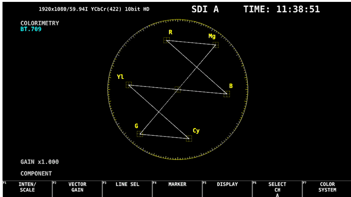
Figure 10-1 Vector display
