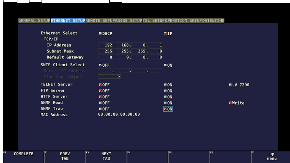
Figure 17-11 ETHERNET SETUP tab
