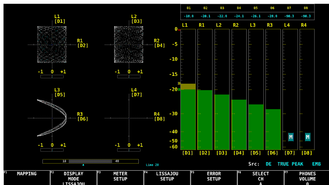
Figure 13-1 Audio display
