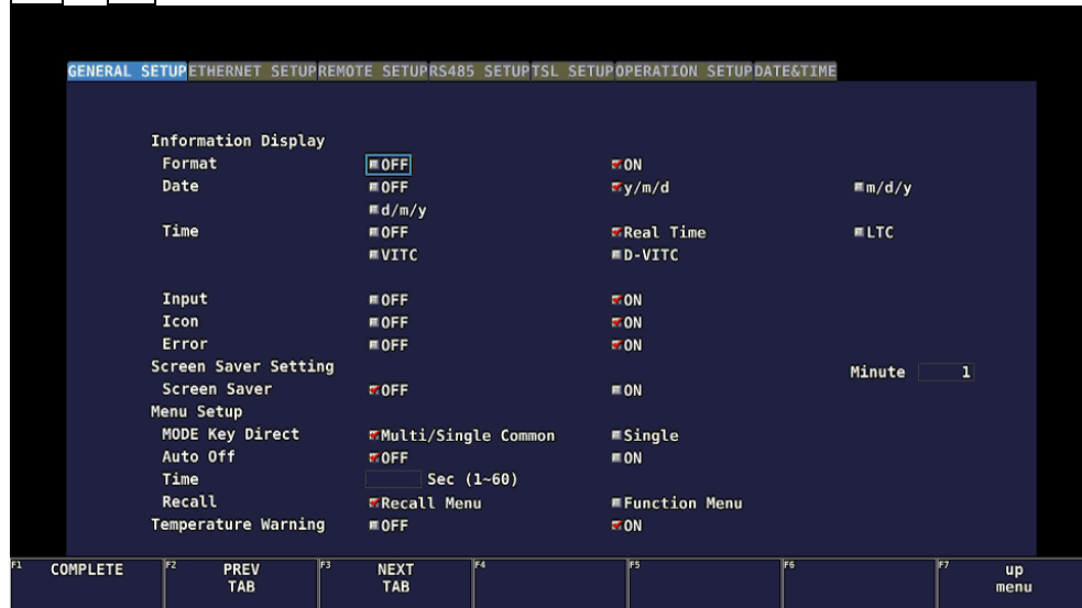
Figure 6-8 GENERAL SETUP tab
