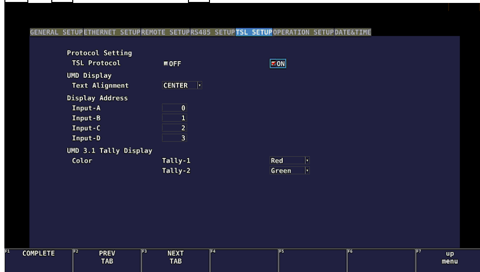
Figure 6-14 TSL SETUP tab
