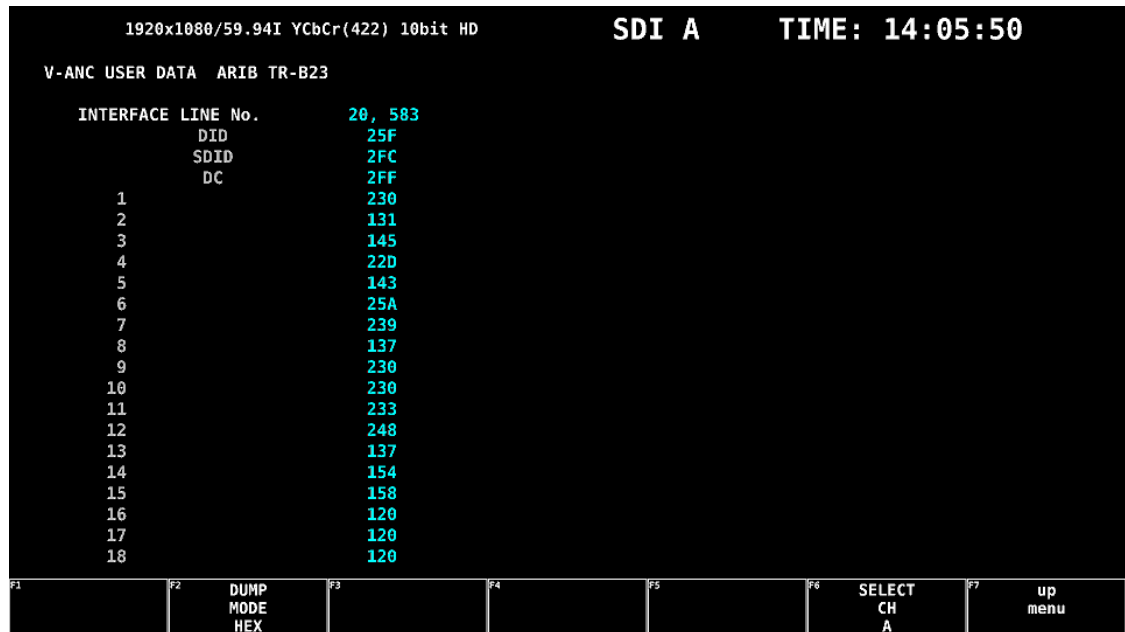
Figure 14-24 User data display
