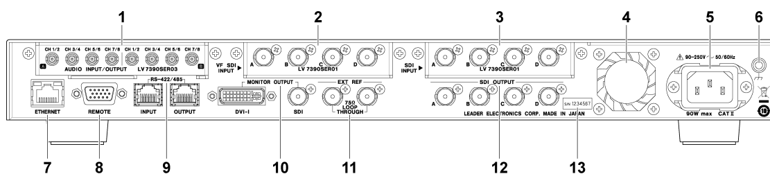
Figure 3-2 Rear panel
