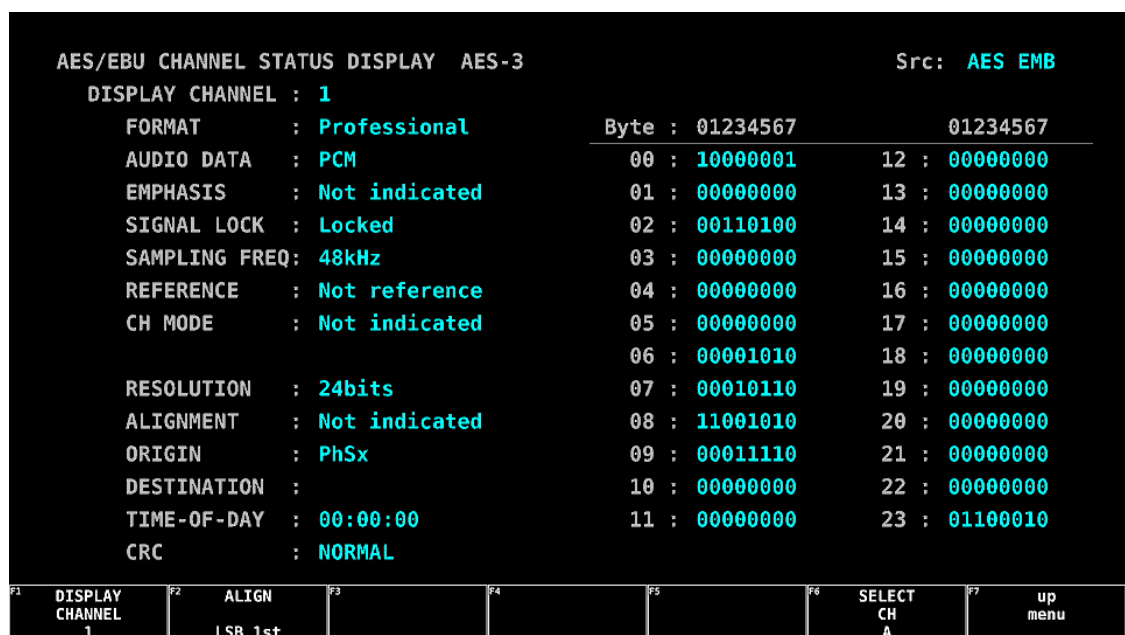
Figure 13-28 Channel status display
