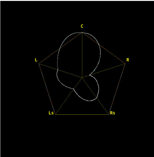
SURROUND 5.1 = NORMAL
