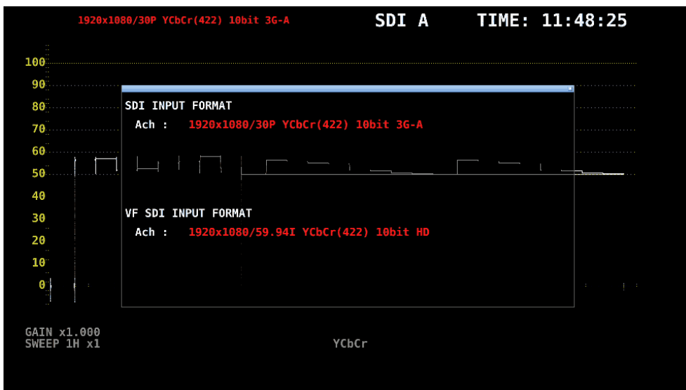
Figure 5-2 Input Format Error Display
