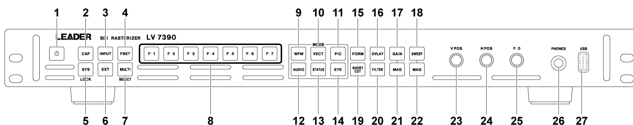
Figure 3-1 Front panel
