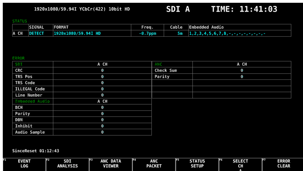
Figure 5-22 Status display
