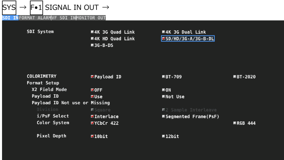
Figure 5-42 SDI IN tab
