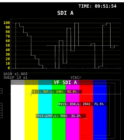
Figure 4-4 Viewfinder display screen
