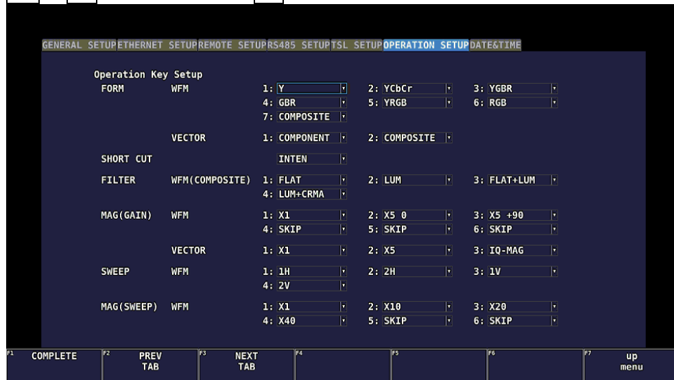
Figure 6-15 OPERATION SETUP tab
