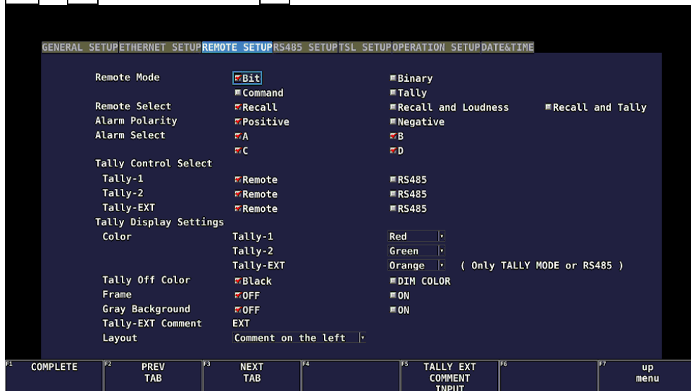
Figure 6-10 REMOTE SETUP tab
