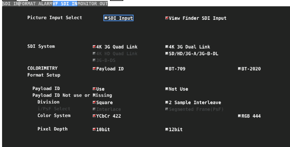
Figure 6-4 VF SDI IN tab
