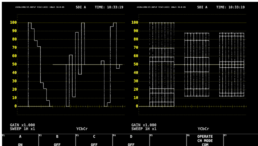
Figure 5-8 Measurement screen
