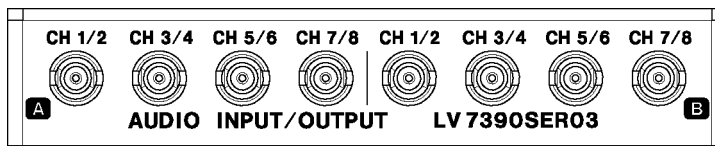
Figure 4-8 Audio I/O connectors
