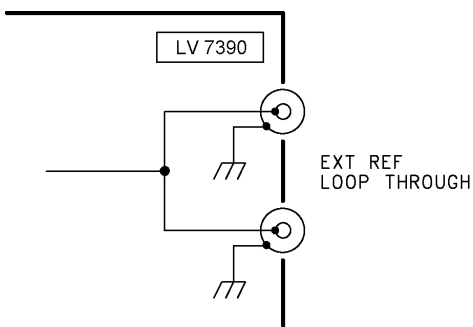
Figure 4-7 Loop-through
