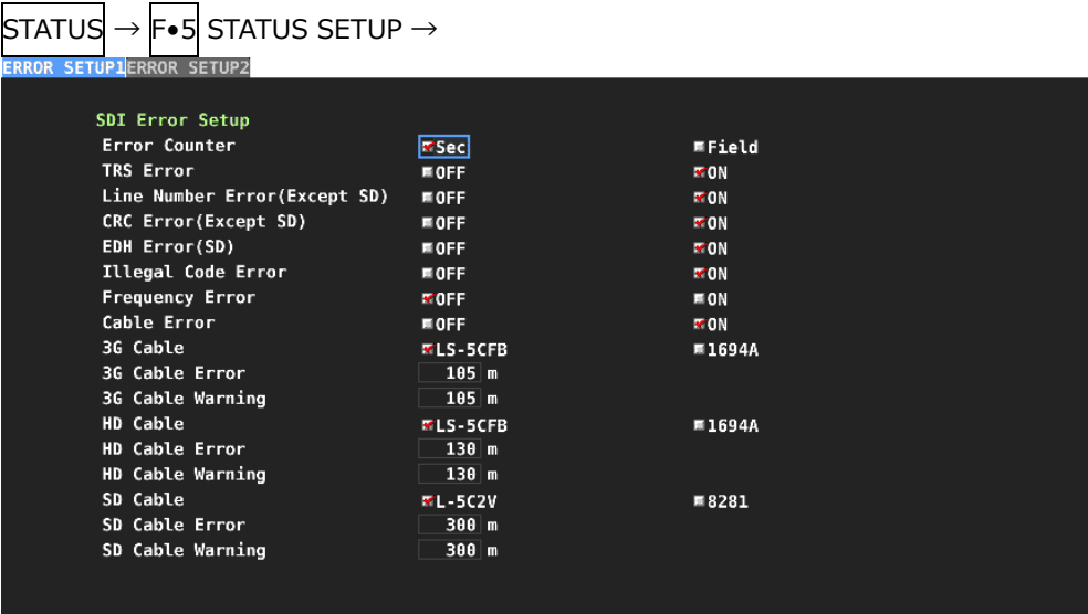
Figure 14-2 ERROR SETUP1 tab
