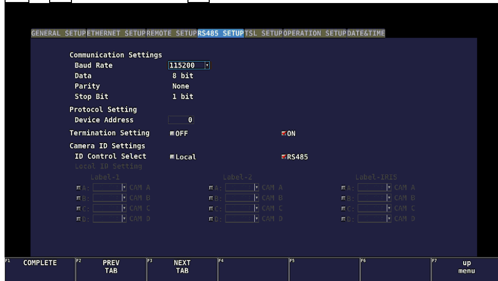
Figure 6-12 RS485 SETUP tab
