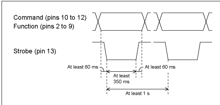
Figure 18-5 Control timing
