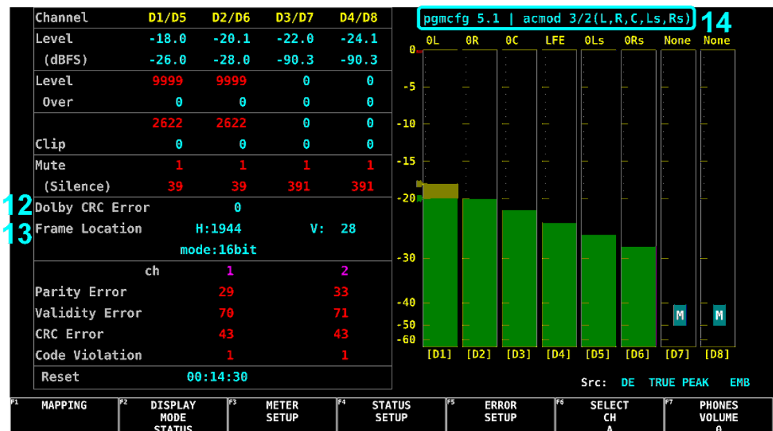
Figure 13-19 Status display (during Dolby measurement)
