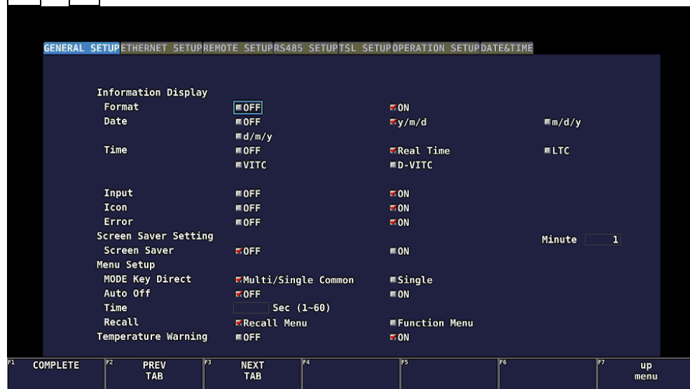
Figure 17-1 GENERAL SETUP tab
