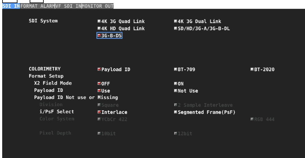
Figure 5-6 SDI IN tab
