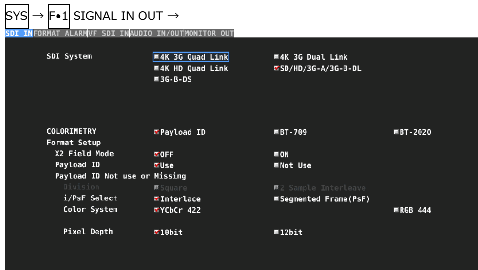
Figure 6-2 SDI IN tab
