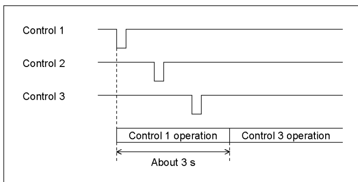
Figure 18-4 Control timing 2
