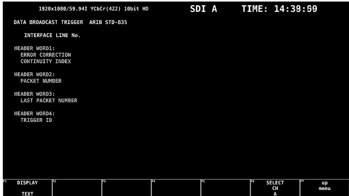
Figure 14-23 Data broadcast trigger signal screen
