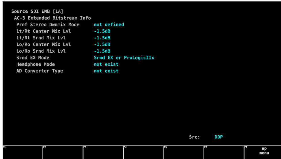
Figure 13-27 Dolby Digital Plus EBI Metadata display
