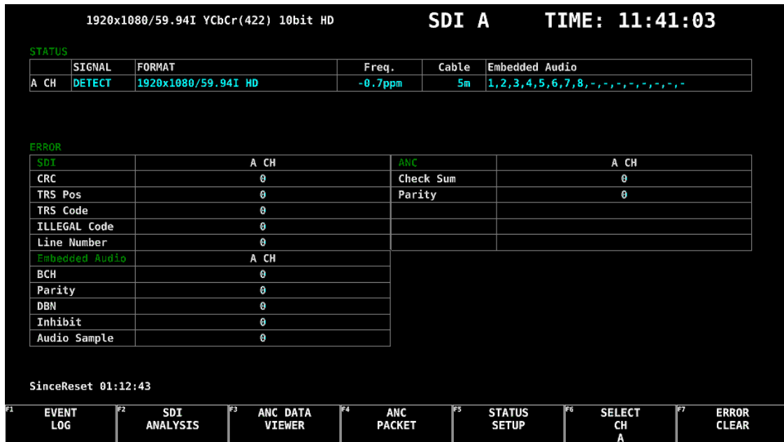
Figure 14-1 Status display
