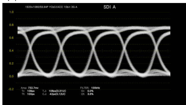
Eye pattern
